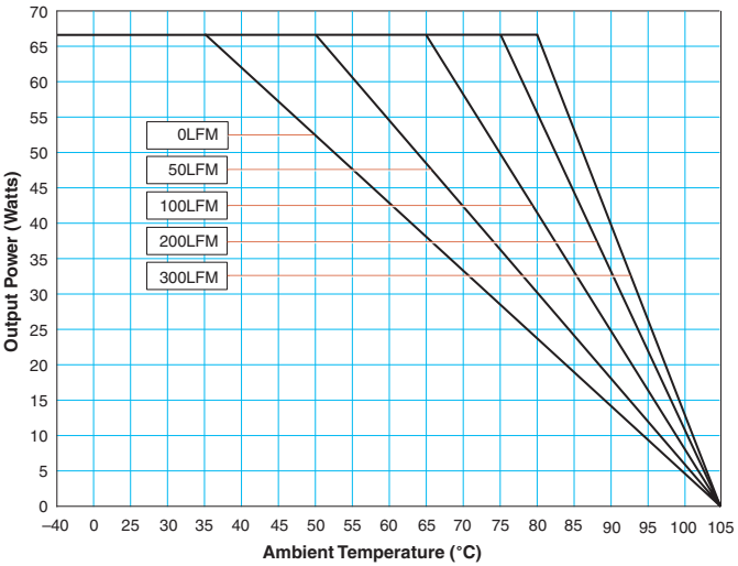
UNR-3.3/20-D5 Output Power Derating vs. Ambient Temperature
