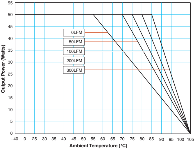
UNR-3.3/15-D5 Output Power Derating vs. Ambient Temperature
