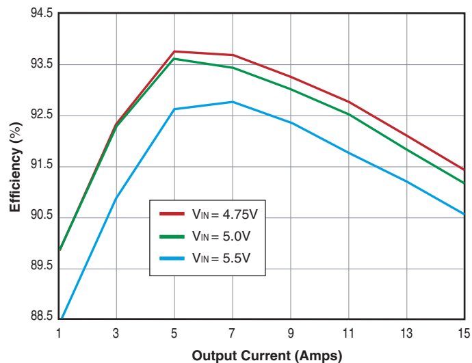
UNR-2.5/15-D5 Efficiency vs. Load @ 25°C Ambient
