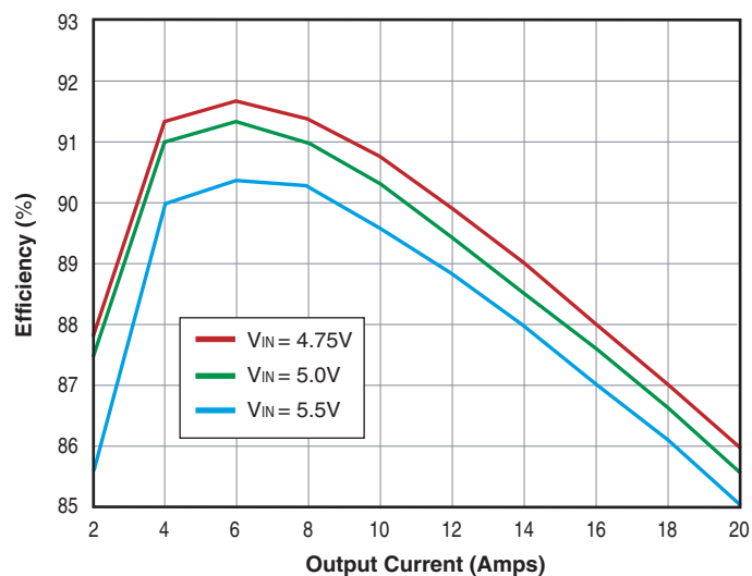
UNR-2.5/20-D5 Efficiency vs. Load @ 25°C Ambient
