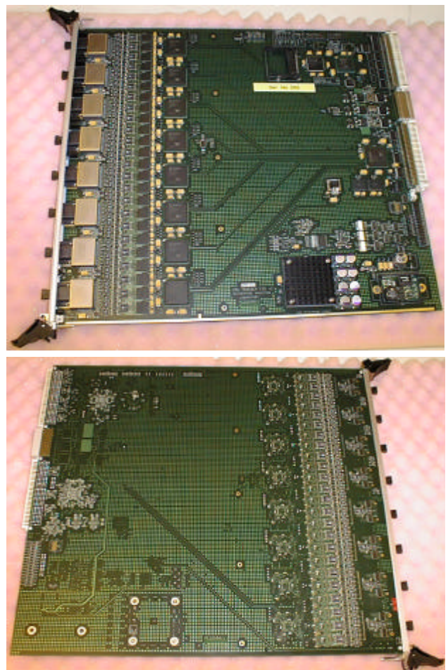
Figure 1: The FEDv1 board primary and secondary sides.
