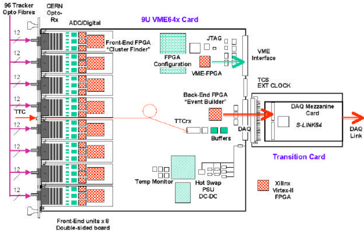
Figure 2: 9U FED board layout with DAQ transition card.
